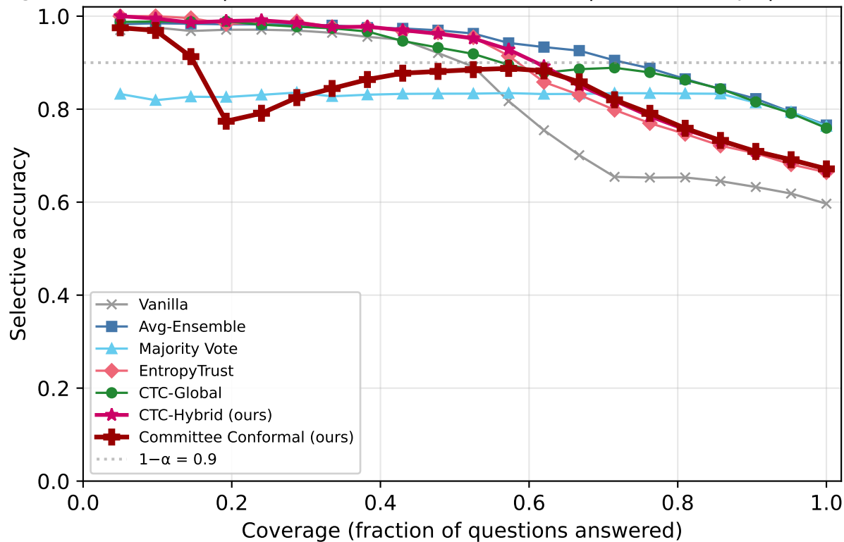
Risk-Coverage: TRUTHFULQA | Qwen3-30B-A3B-Instruct-2507 | k=1/5 corrupt | overconfident_extreme
