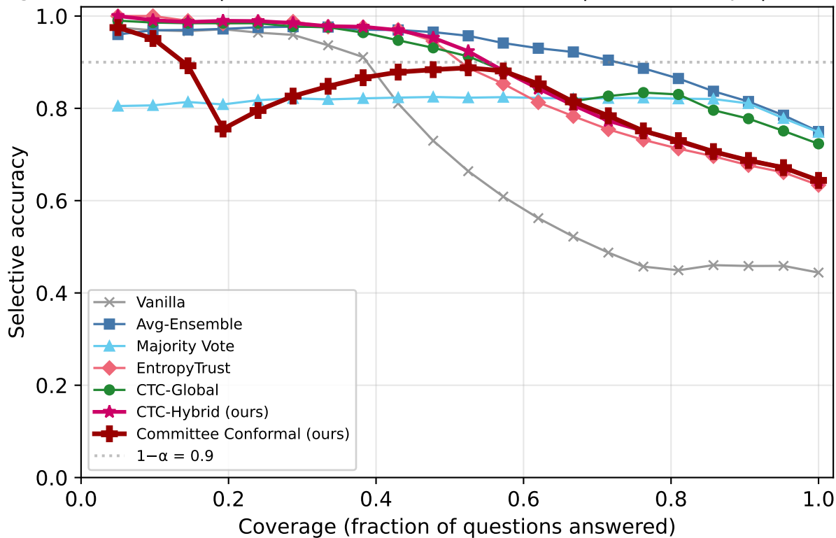
Risk-Coverage: TRUTHFULQA | Qwen3-30B-A3B-Instruct-2507 | k=2/5 corrupt | overconfident_extreme
