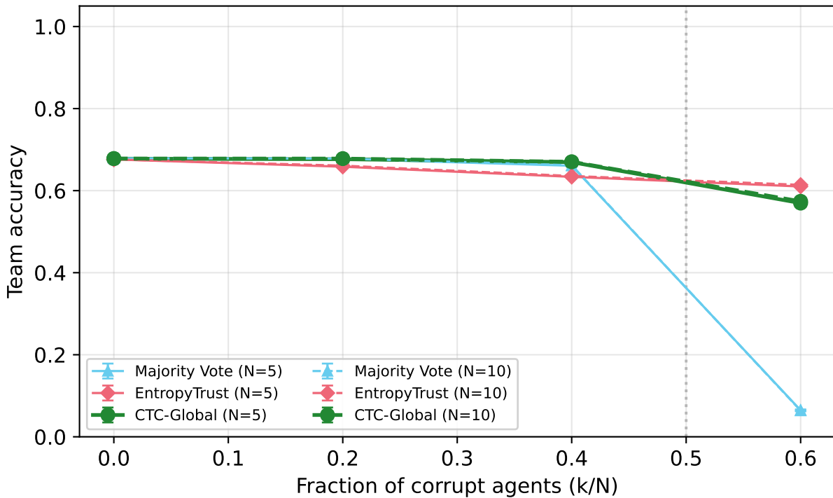
Scaling: N=5 vs N=10 — MMLU (Qwen2.5-7B-Instruct)
