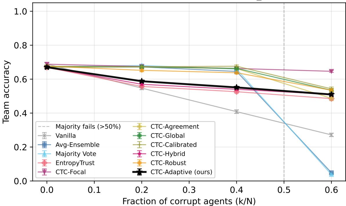
ARC — Mistral-7B-Instruct-v0.3 (overconfident_extreme, \alpha=0.1 )
