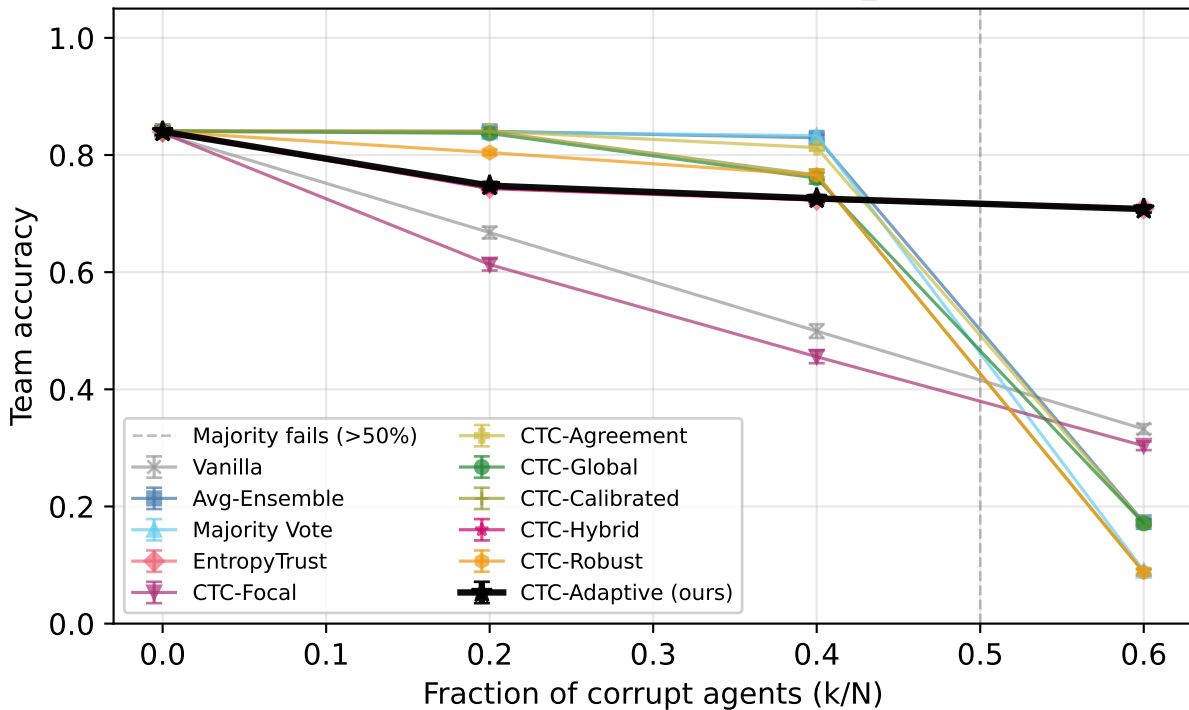
ARC — Phi-3.5-mini-instruct (overconfident_extreme, \alpha=0.1 )
