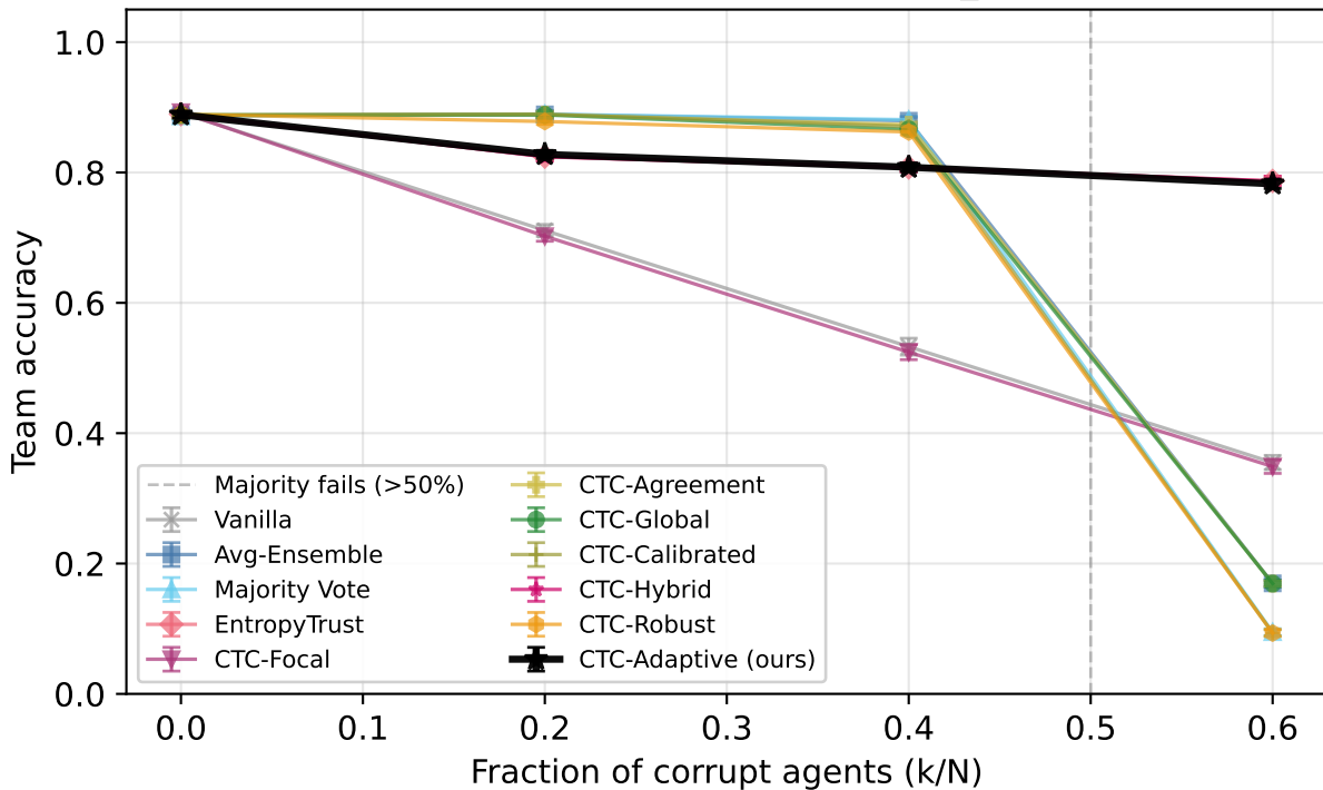
ARC — Qwen2.5-7B-Instruct (overconfident_extreme, \alpha=0.1 )
