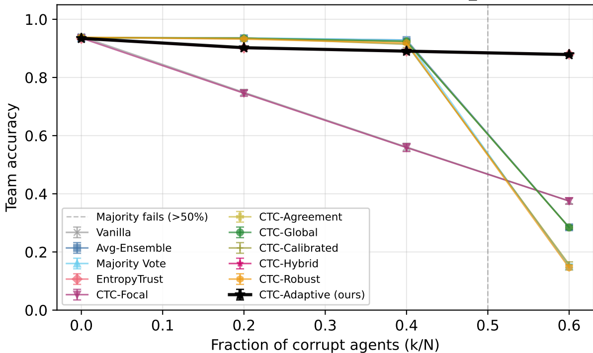
ARC — Qwen3-30B-A3B-Instruct-2507 (overconfident_extreme, \alpha=0.1 )
