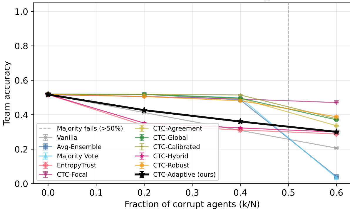
MMLU — Mistral-7B-Instruct-v0.3 (overconfident_extreme, \alpha=0.1 )
