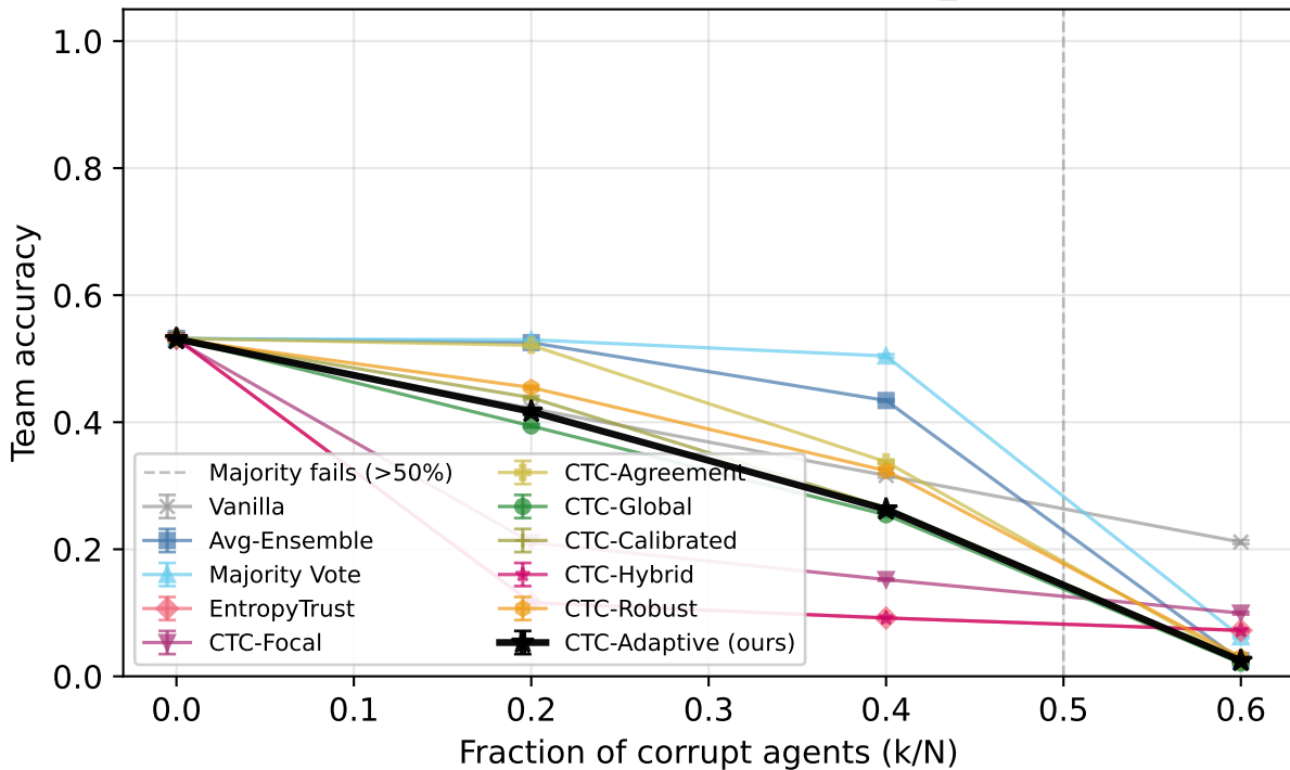
MMLU — Olmo-3-7B-Instruct (overconfident_extreme, \alpha=0.1 )
