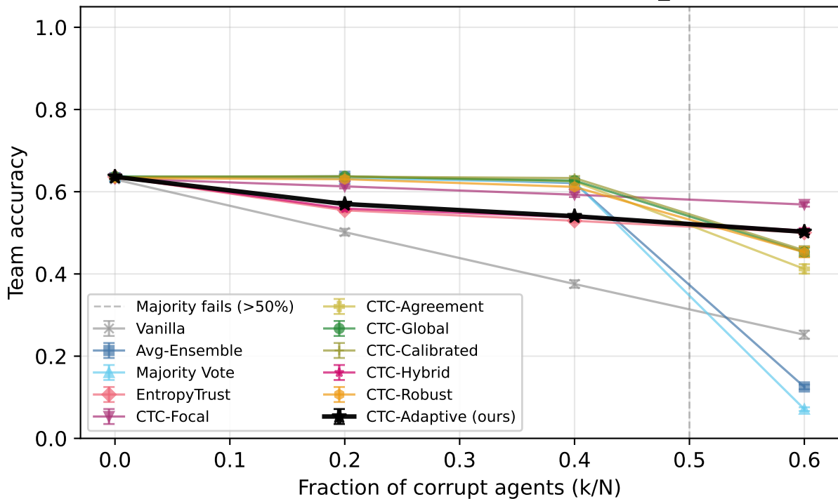
TRUTHFULQA — Phi-3.5-mini-instruct (overconfident_extreme, \alpha=0.1 )
