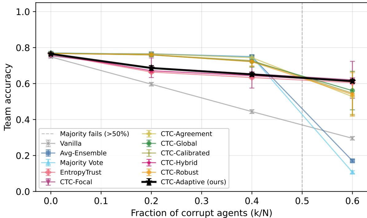
TRUTHFULQA — Qwen3-30B-A3B-Instruct-2507 (overconfident_extreme, \alpha=0.1 )
