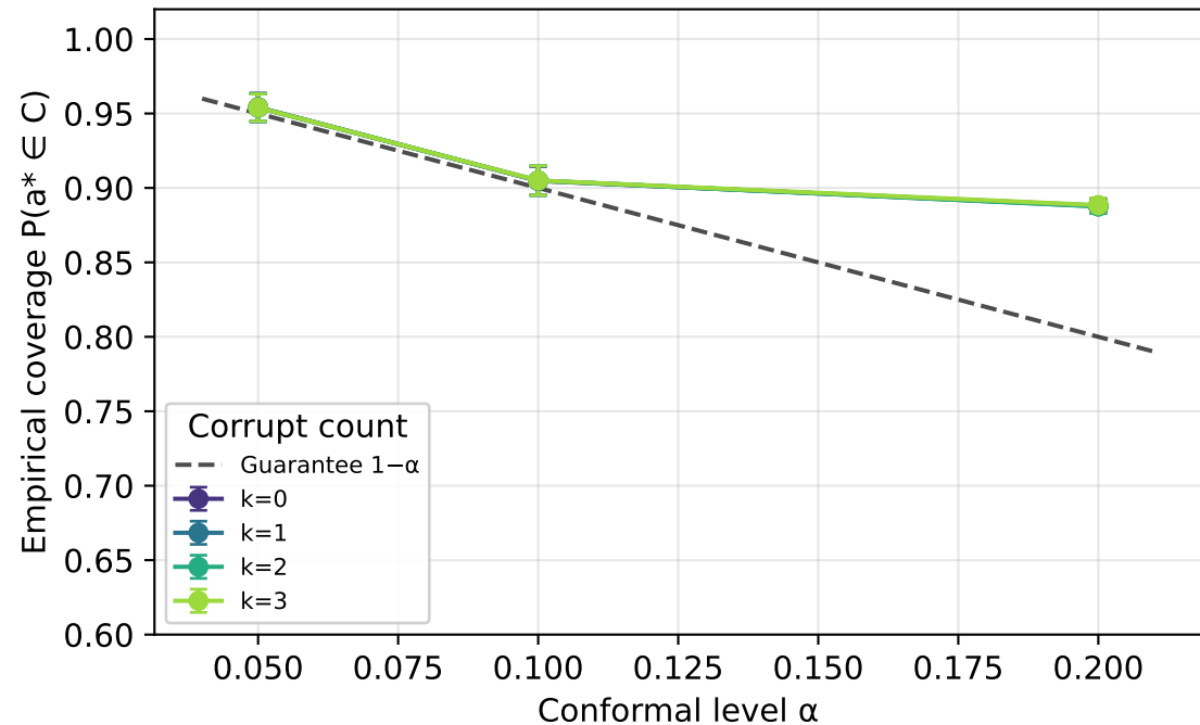
Coverage guarantee — ARC (Qwen2.5-7B-Instruct)
