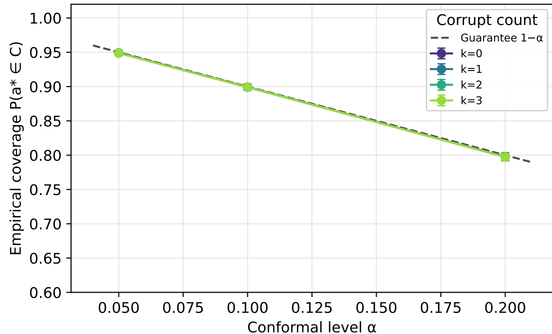
Coverage guarantee — MMLU (Qwen2.5-7B-Instruct)
