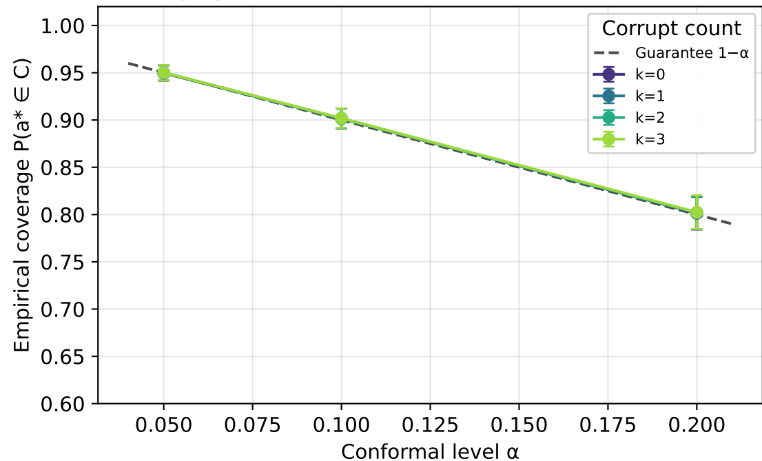
Coverage guarantee — TRUTHFULQA (Qwen2.5-7B-Instruct)
