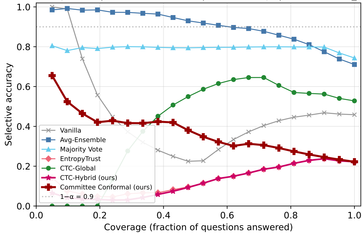
Risk-Coverage: ARC | Olmo-3-7B-Instruct | k=2/5 corrupt | overconfident_extreme
