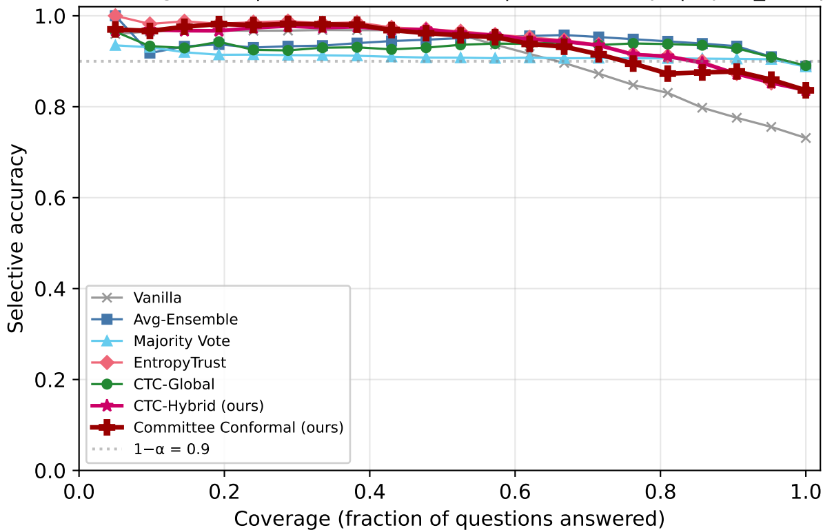
Risk-Coverage: ARC | Qwen2.5-7B-Instruct | k=1/5 corrupt | inject_deceptive
