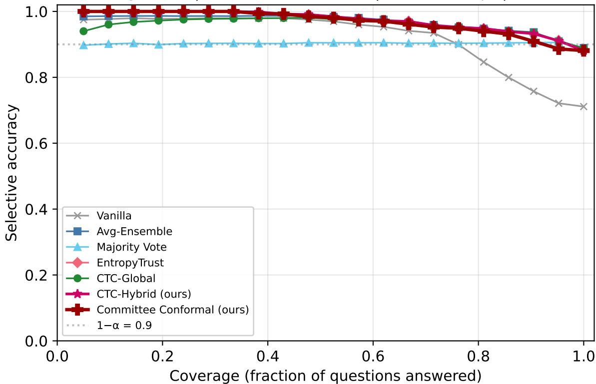
Risk-Coverage: ARC | Qwen2.5-7B-Instruct | k=1/5 corrupt | overconfident
