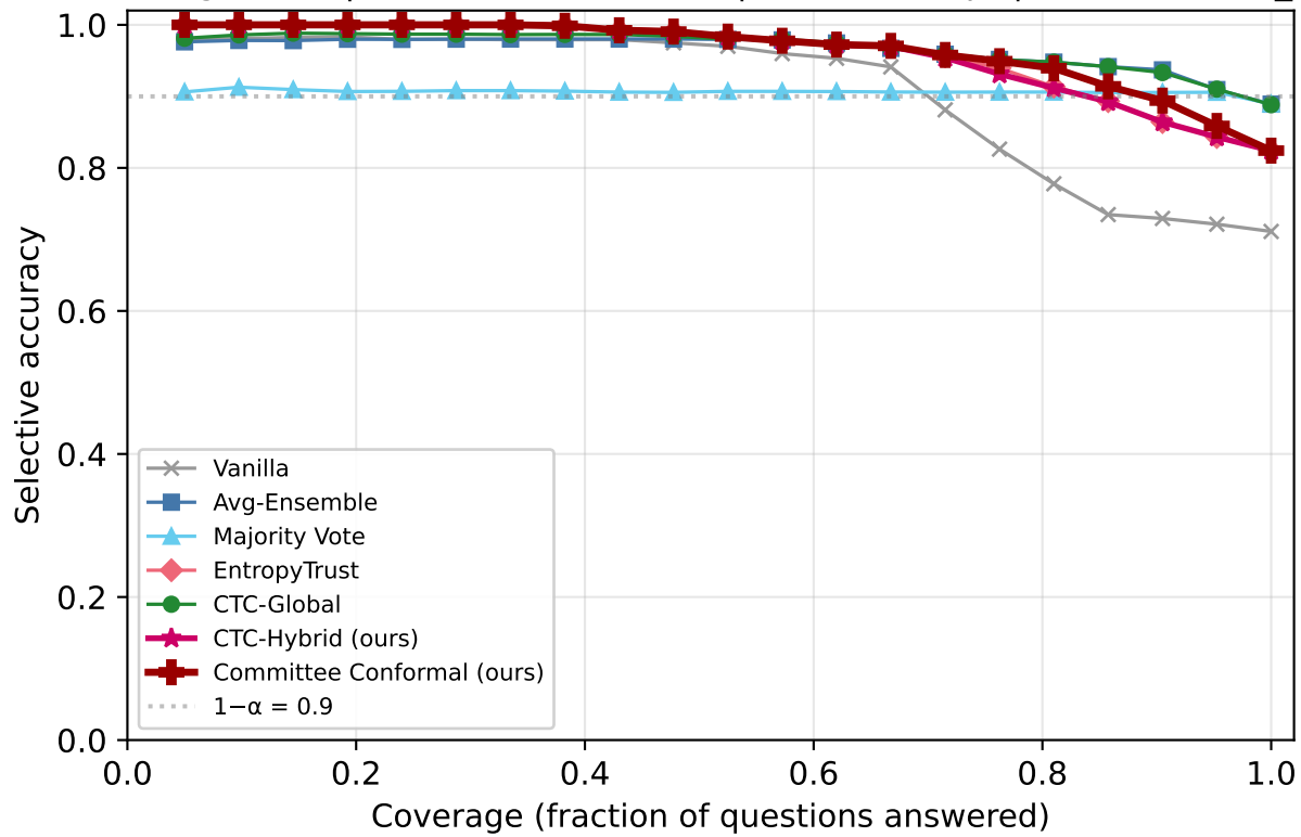
Risk-Coverage: ARC | Qwen2.5-7B-Instruct | k=1/5 corrupt | overconfident_extreme
