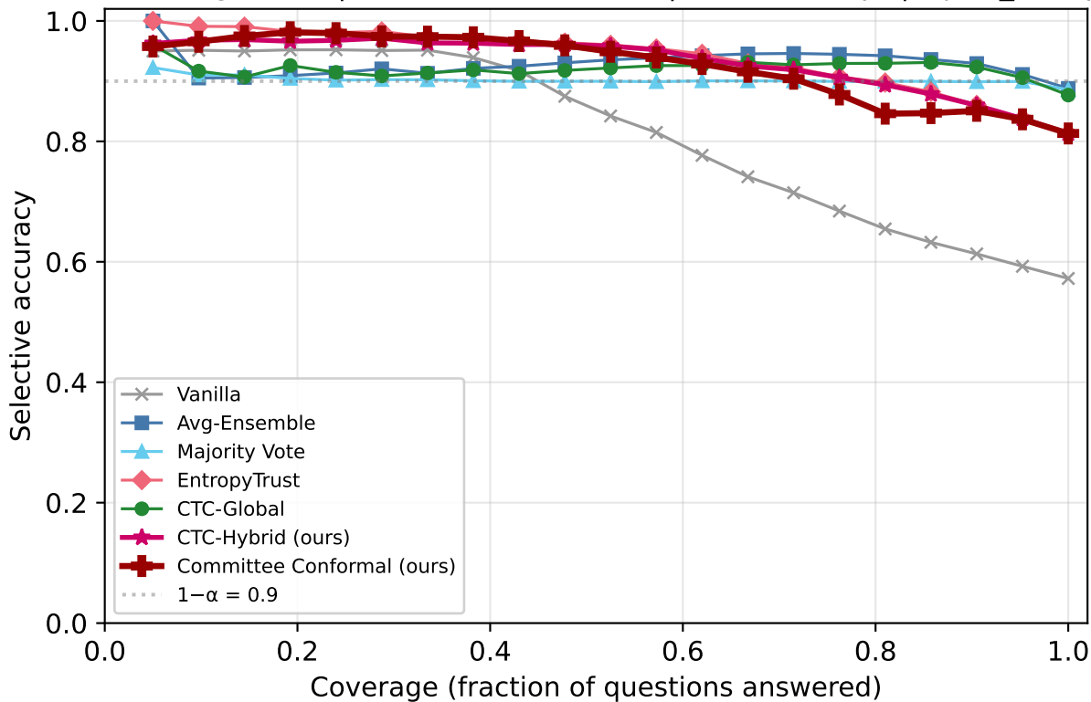
Risk-Coverage: ARC | Qwen2.5-7B-Instruct | k=2/5 corrupt | inject_deceptive
