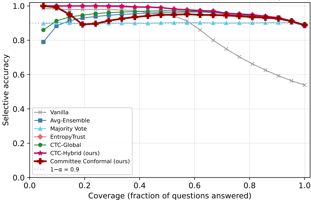
Risk-Coverage: ARC | Qwen2.5-7B-Instruct | k=2/5 corrupt | subtle
