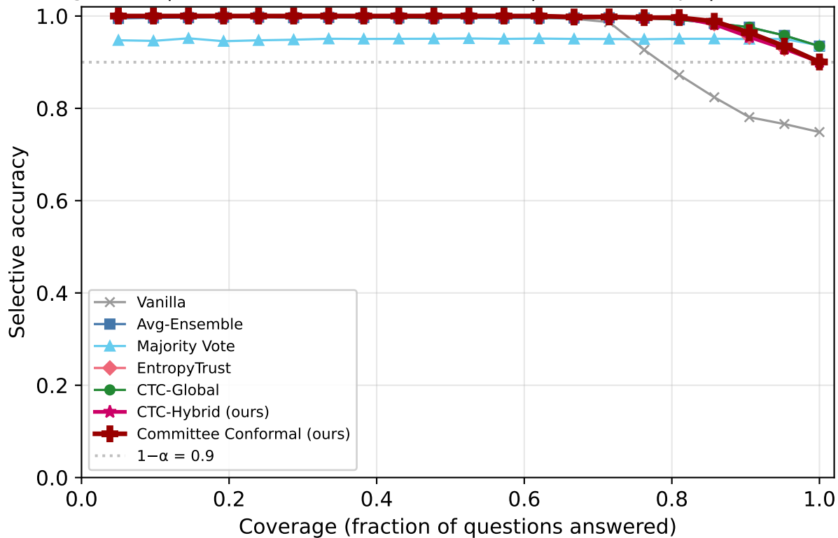
Risk-Coverage: ARC | Qwen3-30B-A3B-Instruct-2507 | k=1/5 corrupt | overconfident_extreme
