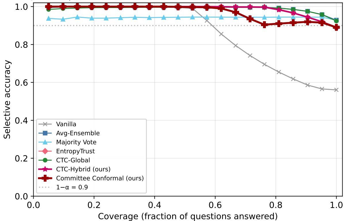
Risk-Coverage: ARC | Qwen3-30B-A3B-Instruct-2507 | k=2/5 corrupt | overconfident_extreme
