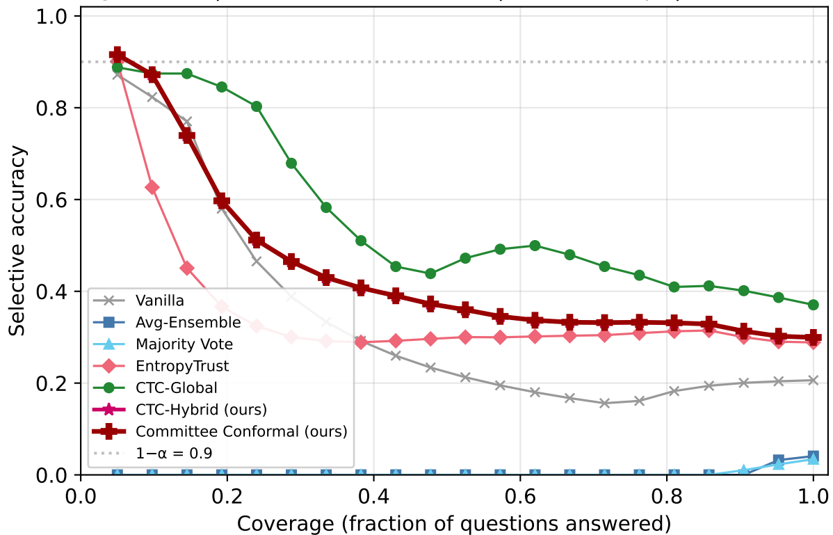
Risk-Coverage: MMLU | Mistral-7B-Instruct-v0.3 | k=3/5 corrupt | overconfident_extreme
