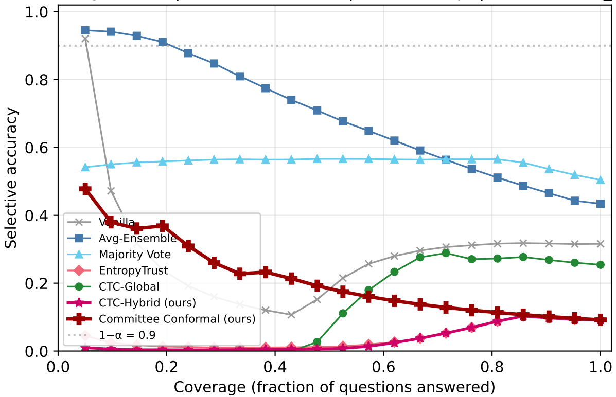
Risk-Coverage: MMLU | Olmo-3-7B-Instruct | k=2/5 corrupt | overconfident_extreme
