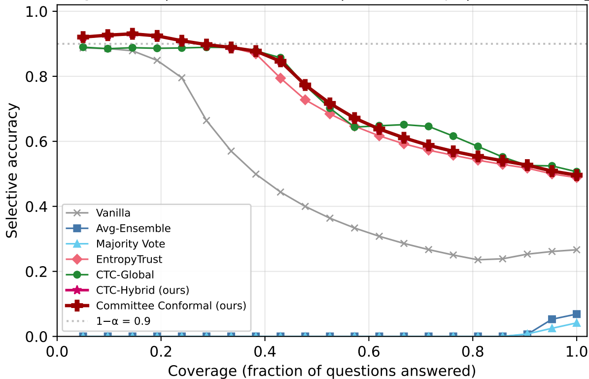
Risk-Coverage: MMLU | Phi-3.5-mini-instruct | k=3/5 corrupt | overconfident_extreme
