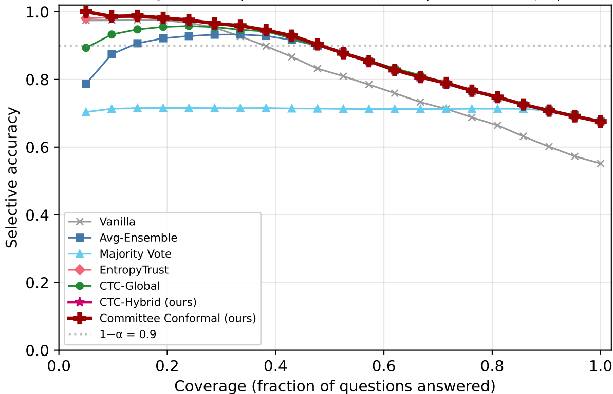
Risk-Coverage: MMLU | Qwen2.5-7B-Instruct | k=1/5 corrupt | subtle
