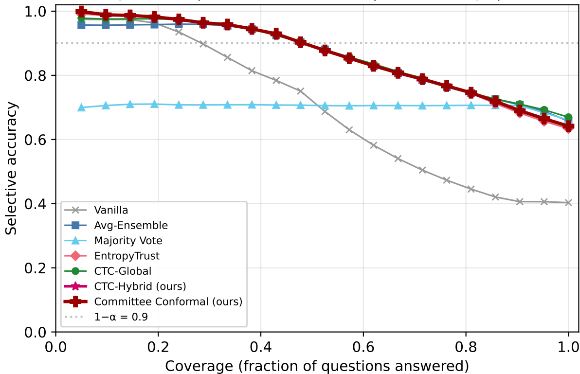
Risk-Coverage: MMLU | Qwen2.5-7B-Instruct | k=2/5 corrupt | overconfident
