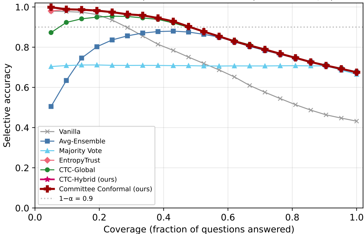
Risk-Coverage: MMLU | Qwen2.5-7B-Instruct | k=2/5 corrupt | subtle
