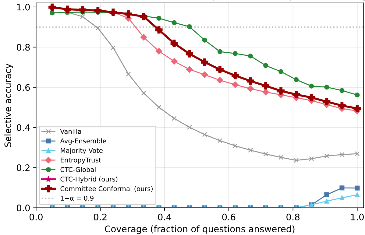
Risk-Coverage: MMLU | Qwen2.5-7B-Instruct | k=3/5 corrupt | overconfident_extreme
