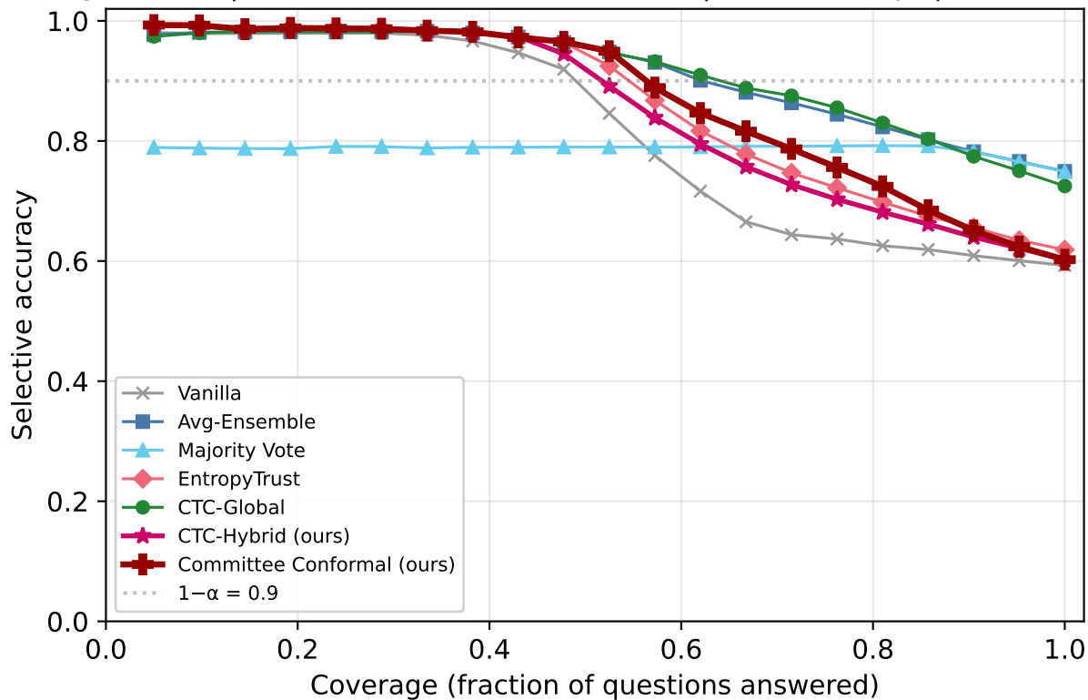
Risk-Coverage: MMLU | Qwen3-30B-A3B-Instruct-2507 | k=1/5 corrupt | overconfident_extreme
