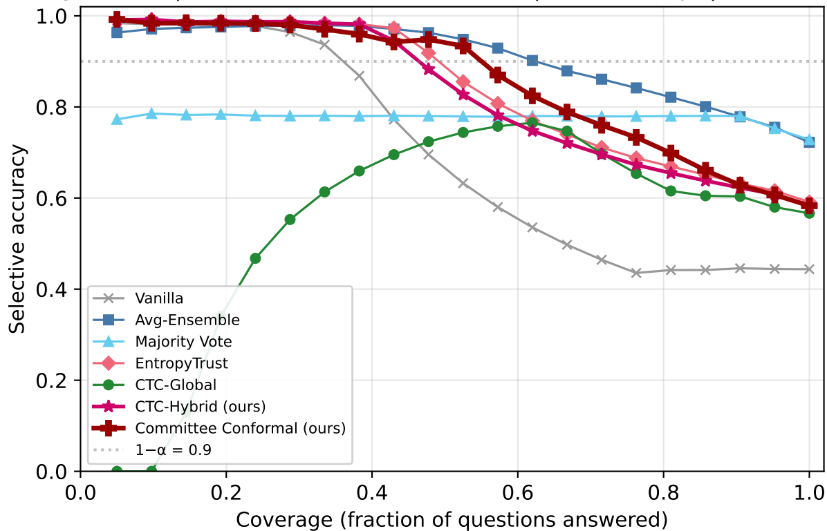
Risk-Coverage: MMLU | Qwen3-30B-A3B-Instruct-2507 | k=2/5 corrupt | overconfident_extreme
