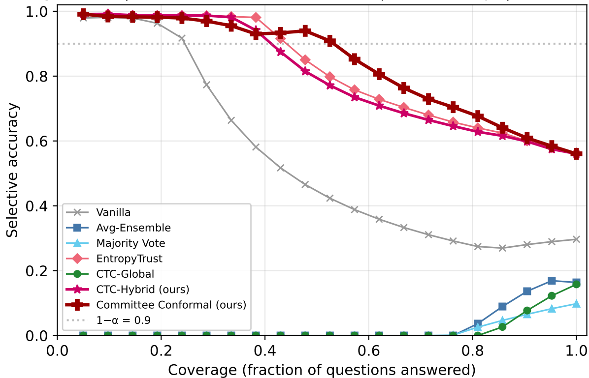
Risk-Coverage: MMLU | Qwen3-30B-A3B-Instruct-2507 | k=3/5 corrupt | overconfident_extreme
