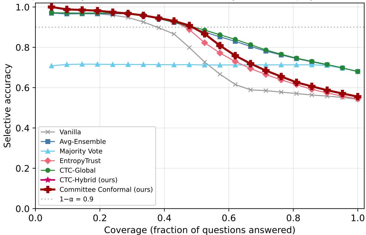
Risk-Coverage: MMLU | domain:Qwen2.5-7B-Instruct | k=1/5 corrupt | overconfident_extreme
