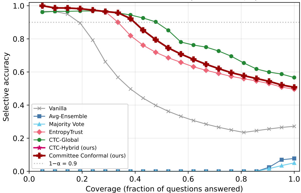
Risk-Coverage: MMLU | domain:Qwen2.5-7B-Instruct | k=3/5 corrupt | overconfident_extreme
