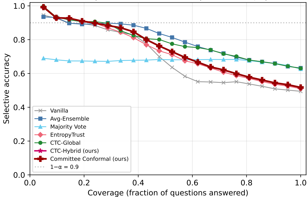
Risk-Coverage: TRUTHFULQA | Mistral-7B-Instruct-v0.3 | k=1/5 corrupt | overconfident_extreme
