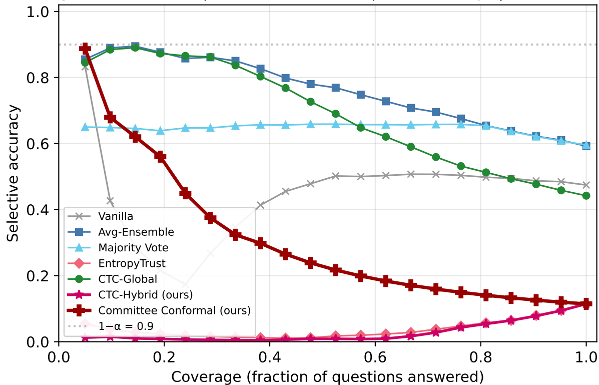
Risk-Coverage: TRUTHFULQA | Olmo-3-7B-Instruct | k=1/5 corrupt | overconfident_extreme
