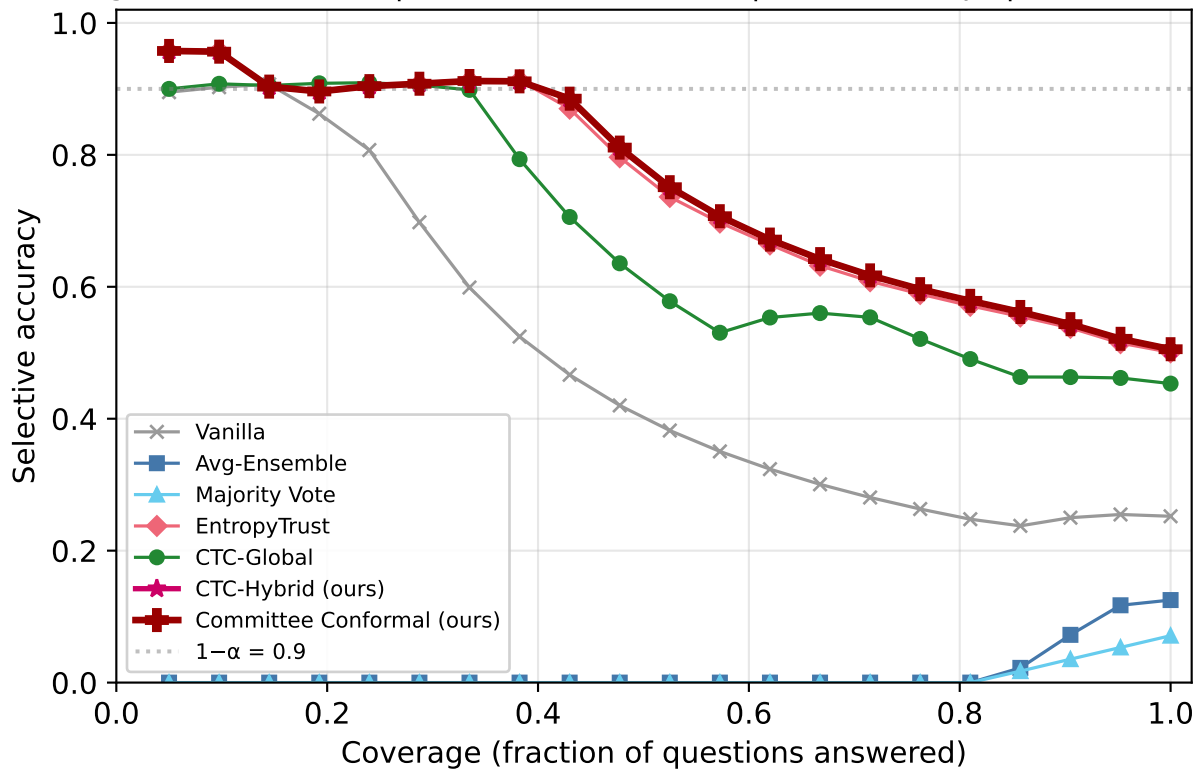
Risk-Coverage: TRUTHFULQA | Phi-3.5-mini-instruct | k=3/5 corrupt | overconfident_extreme
