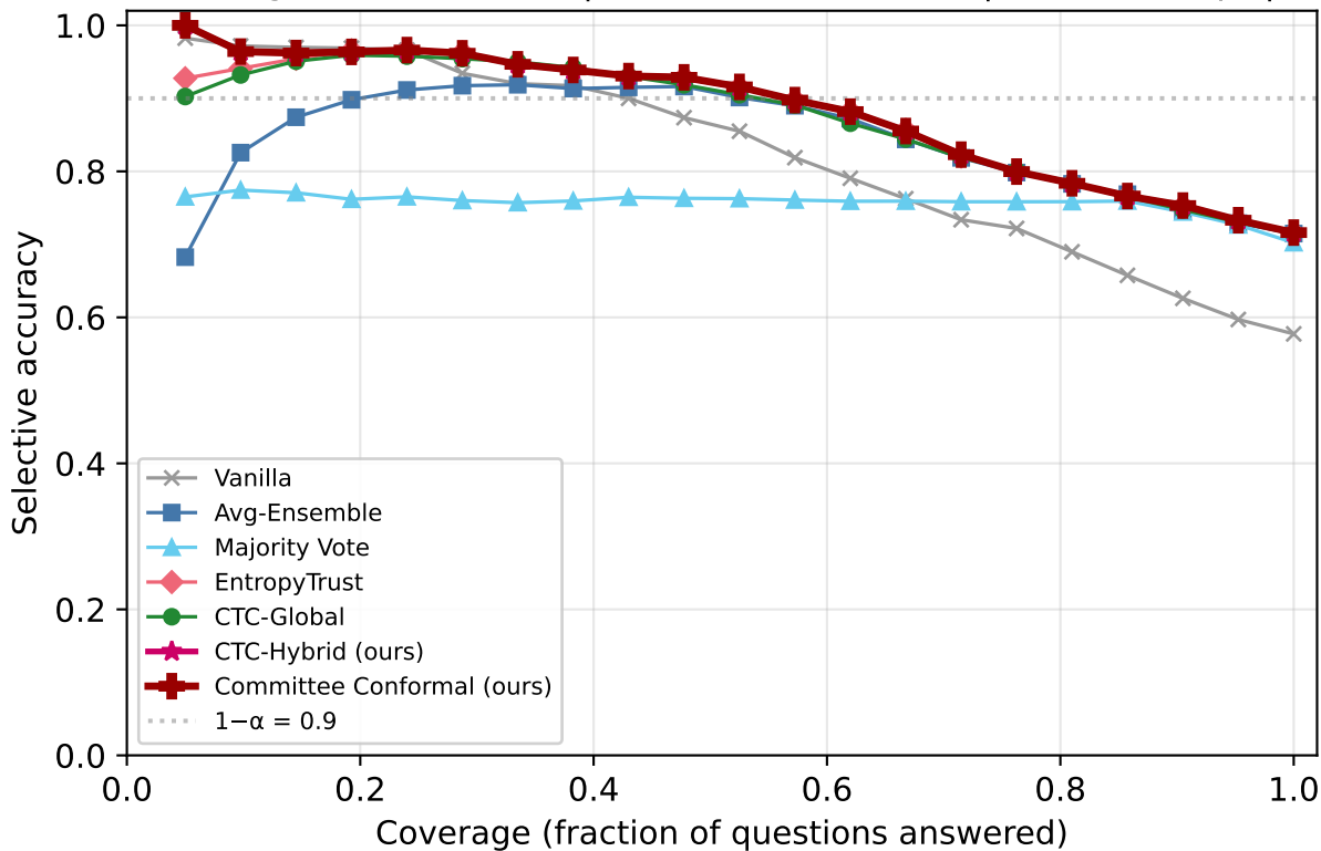
Risk-Coverage: TRUTHFULQA | Qwen2.5-7B-Instruct | k=1/5 corrupt | subtle
