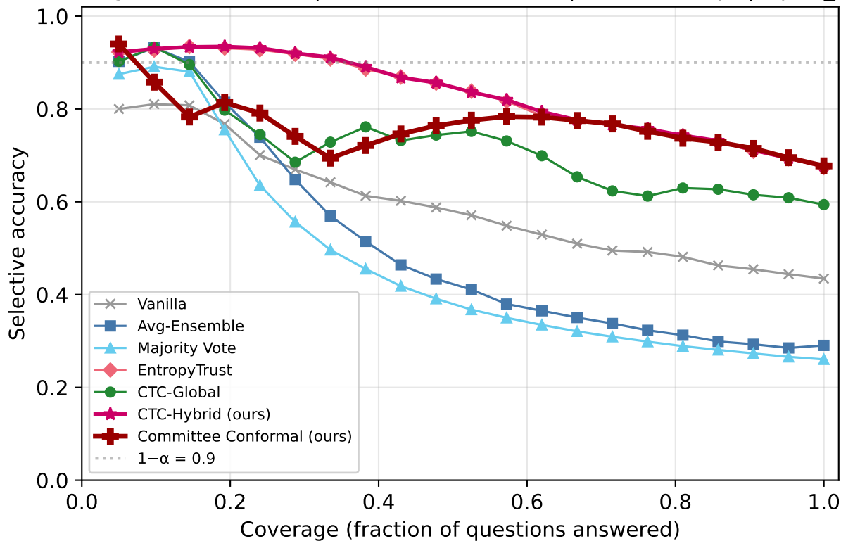
Risk-Coverage: TRUTHFULQA | Qwen2.5-7B-Instruct | k=3/5 corrupt | inject_deceptive
