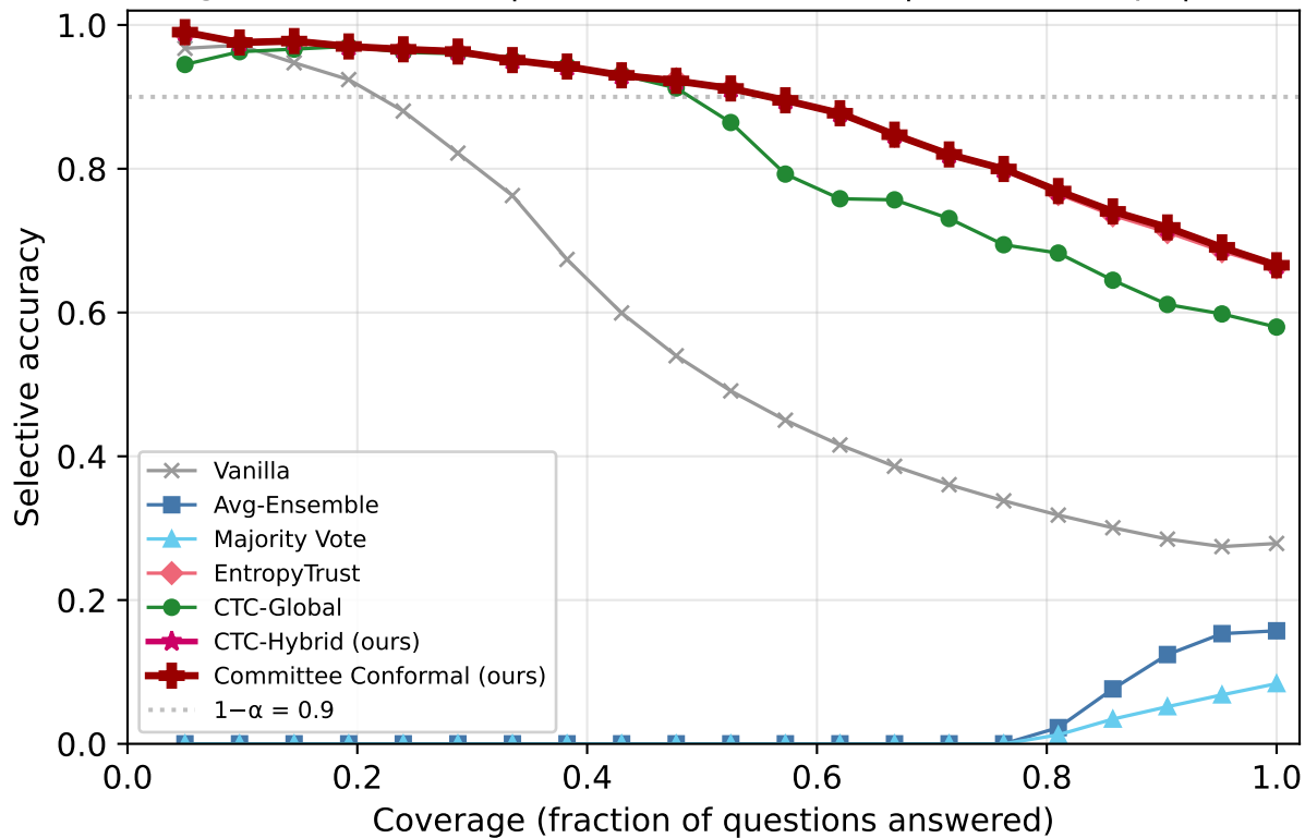
Risk-Coverage: TRUTHFULQA | Qwen2.5-7B-Instruct | k=3/5 corrupt | overconfident
