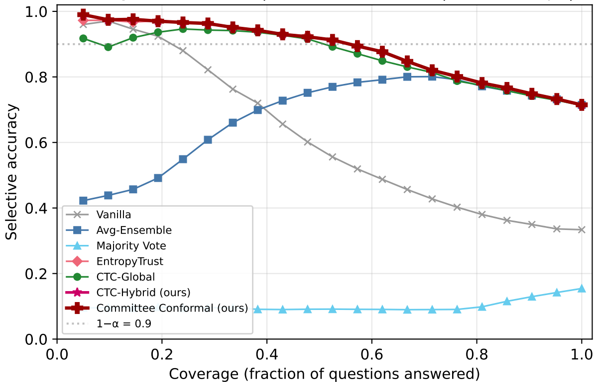
Risk-Coverage: TRUTHFULQA | Qwen2.5-7B-Instruct | k=3/5 corrupt | subtle
