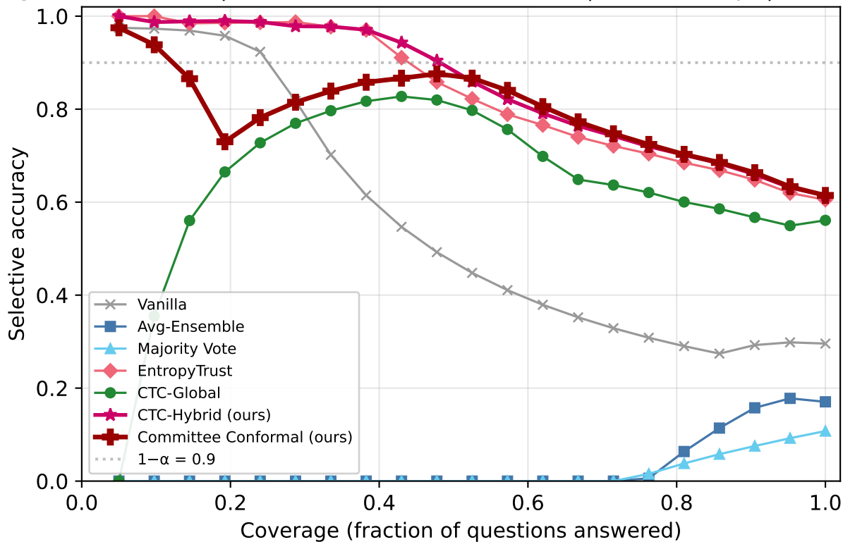
Risk-Coverage: TRUTHFULQA | Qwen3-30B-A3B-Instruct-2507 | k=3/5 corrupt | overconfident_extreme
