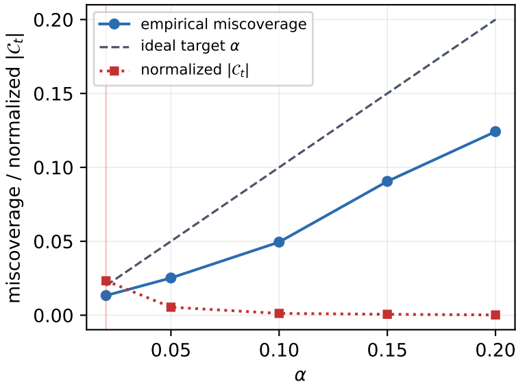
Calibration diagnostics vs. \alpha
