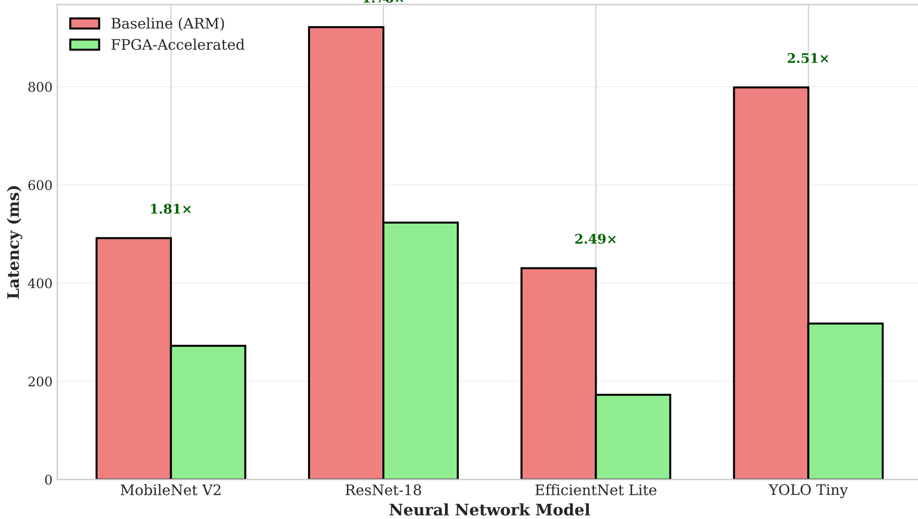
Performance Comparison: Baseline vs FPGA-Accelerated
