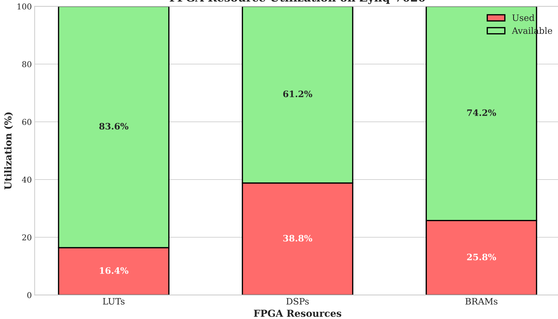
FPGA Resource Utilization on Zynq-7020
