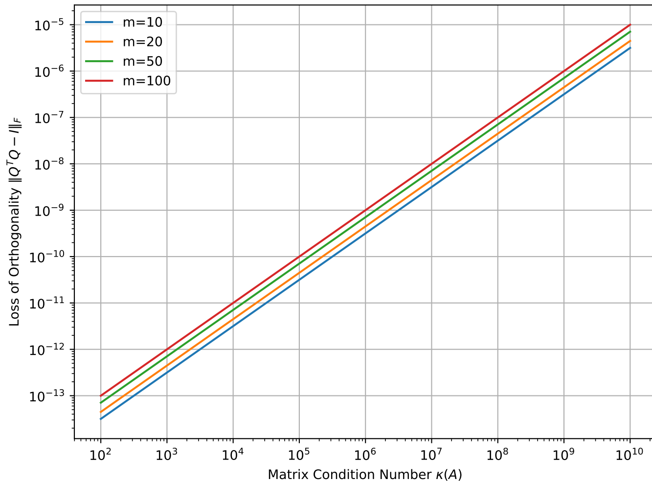
Numerical Stability: \kappa(A) vs Orthogonality Drift
