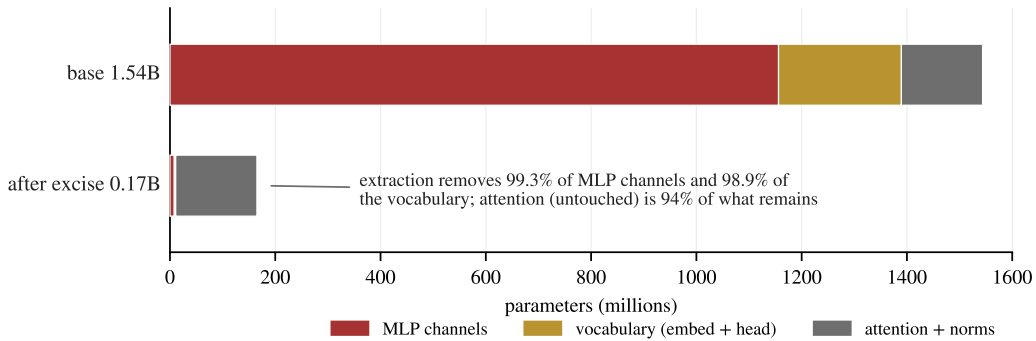
Figure 7: Where the parameters go. Qwen2.5-Math-1.5B before and after extraction at the 0.71% floor: 99.3% of MLP channels and 98.9% of the vocabulary are deleted outright; attention and norms, which the method does not touch, are 94% of what remains — the obvious next structured dimension.
