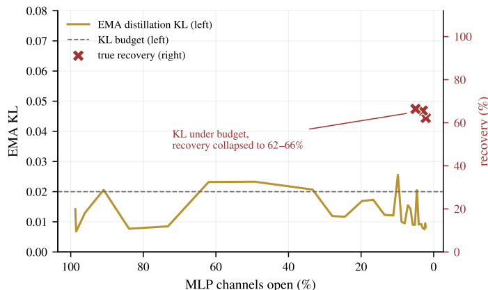
Figure 8: Losses lie; generations don’t. The failed KL-only controller (v2.0): EMA distillation KL stays under budget throughout the descent (left axis) while true held-out recovery collapses (crosses, right axis). Generation probes detect this; losses do not.
