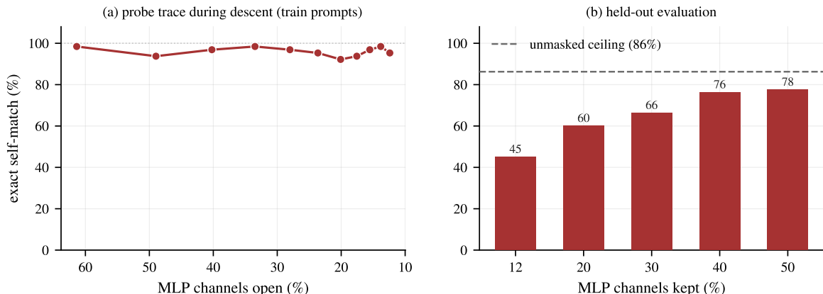
Figure 4: Function calling extracts label-free; data, not machinery, binds generalization. Qwen3-4B. Left: probe trace during descent — exact self-match holds at 92–98% from 61% open down to 12% open on training prompts. Right: held-out self-match by budget; the dashed line is the unmasked adapted model’s own self-match (86%), which upper-bounds every masked number.
