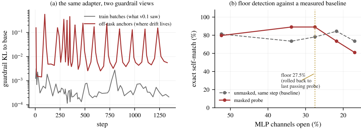
Figure 6: v0.2 calibration in action (JSON extraction run). (a) The guardrail KL measured on train batches (gray) vs. rotating off-task anchor batches (red), same adapter, same steps: the train-batch view—all v0.1 had—reads 10–100× lower than the anchor view. Drift lives exactly where a train-only guardrail cannot see it. (b) Floor detection: the masked probe (red) is compared against the unmasked model measured at the same step (gray, itself depressed by decode noise and residual drift), not against an assumed 100%; when the masked probe falls below tolerance twice, the gates roll back to the last passing sparsity (27.5%).
