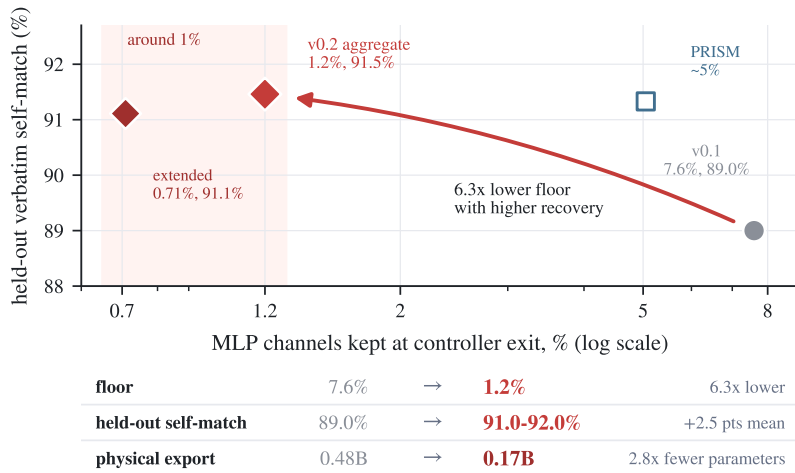
Figure 1: Two-digit addition runs on 0.7–1.2% of MLP channels, found automatically in one label-free run. Qwen2.5-Math-1.5B. The red aggregate marker summarizes three configured lower-bound exits at 1.2% of channels (91.0–92.0% held-out verbatim self-match); the dark red marker is the extended step-cap exit at 0.71%. The x-axis is log-scaled. The blue PRISM point is the reported staged-pipeline reference [13] (task accuracy), shown for context; caveats in §5.
