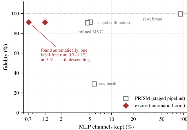
Figure 1: Two-digit addition runs on under 1% of MLP channels, found automatically in one label-free run. Qwen2.5-Math-1.5B. Red diamonds are excise ’s controller stopping points: three configured lower-bound exits at 1.2% of channels and one extended step-cap exit at 0.71%, plotted by held-out verbatim self-match, a stricter metric that lower-bounds recovery. Gray squares are PRISM’s staged pipeline as reported [13] (recovery, task accuracy), shown for reference. Caveats in §5.
