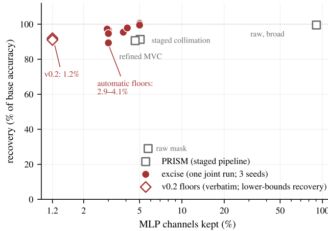
Figure 1: One joint run dominates the staged pipeline. Sparsity–recovery frontier for 2-digit addition on Qwen2.5-Math-1.5B. Gray squares: PRISM’s staged pipeline as reported [13]. Red circles: a single excise run per seed (3 seeds) emits the entire frontier; the floors (2.9–4.1%) were found by the controller, not swept. Open diamonds: the released library’s v0.2 floors (§3.4) — all three seeds at 1.2%, plotted by held-out verbatim self-match, which lower-bounds recovery. Caveats for this comparison in §5.
