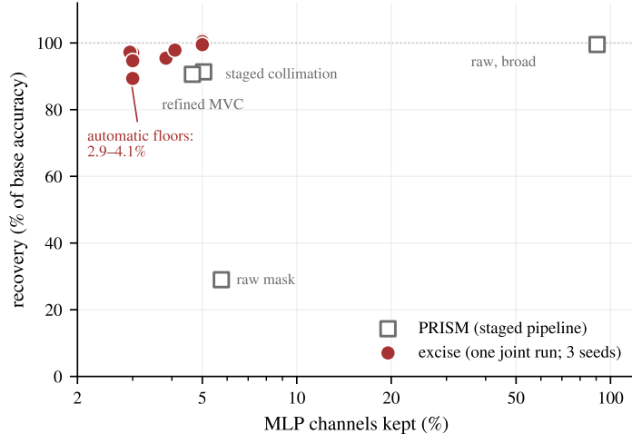
Figure 2: Sparsity–recovery frontier, 2-digit addition, Qwen2.5-Math-1.5B. Gray squares: PRISM’s staged pipeline as reported [12]. Red circles: one excise run per seed (3 seeds), which emits the whole frontier; floors (2.9–4.1%) were found by the controller, not swept. Caveats for this comparison in §5.
