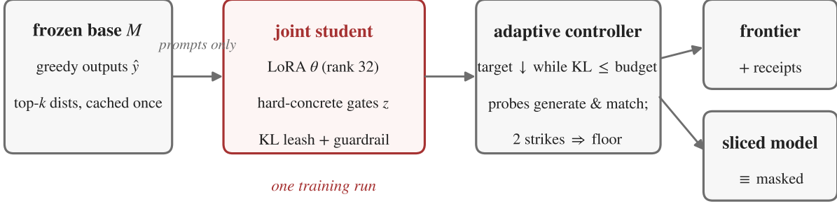
Figure 1: One-shot extraction. The frozen base model supplies label-free targets (greedy outputs and cached top- k distributions); gates and adapter train jointly under a KL leash; an adaptive controller paced by generation probes finds the floor; the run emits the sparsity–fidelity frontier, integrity receipts, and a physically sliced model.
